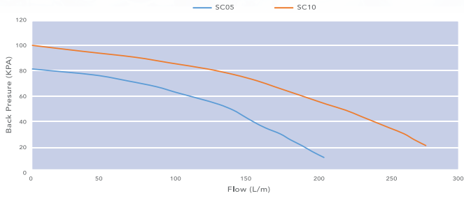
Boost Pump Performance Curves
