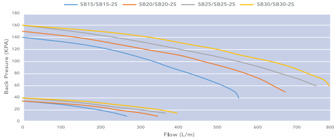
Boost Pump Performance Curves
